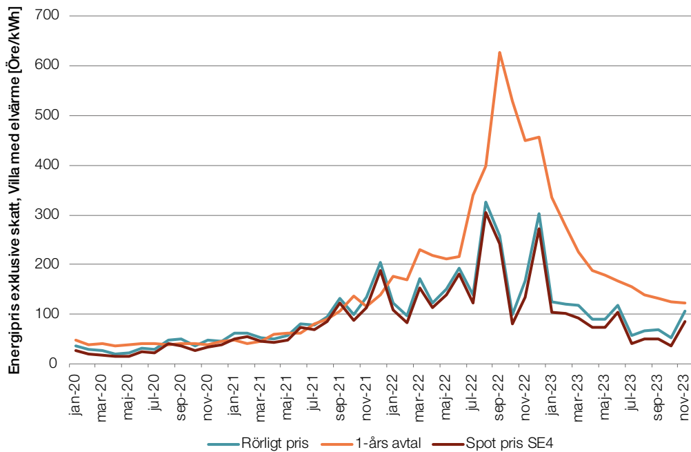
Figur 18 Elhandelspriser i SE4 tom november 2023, öre/kWh
